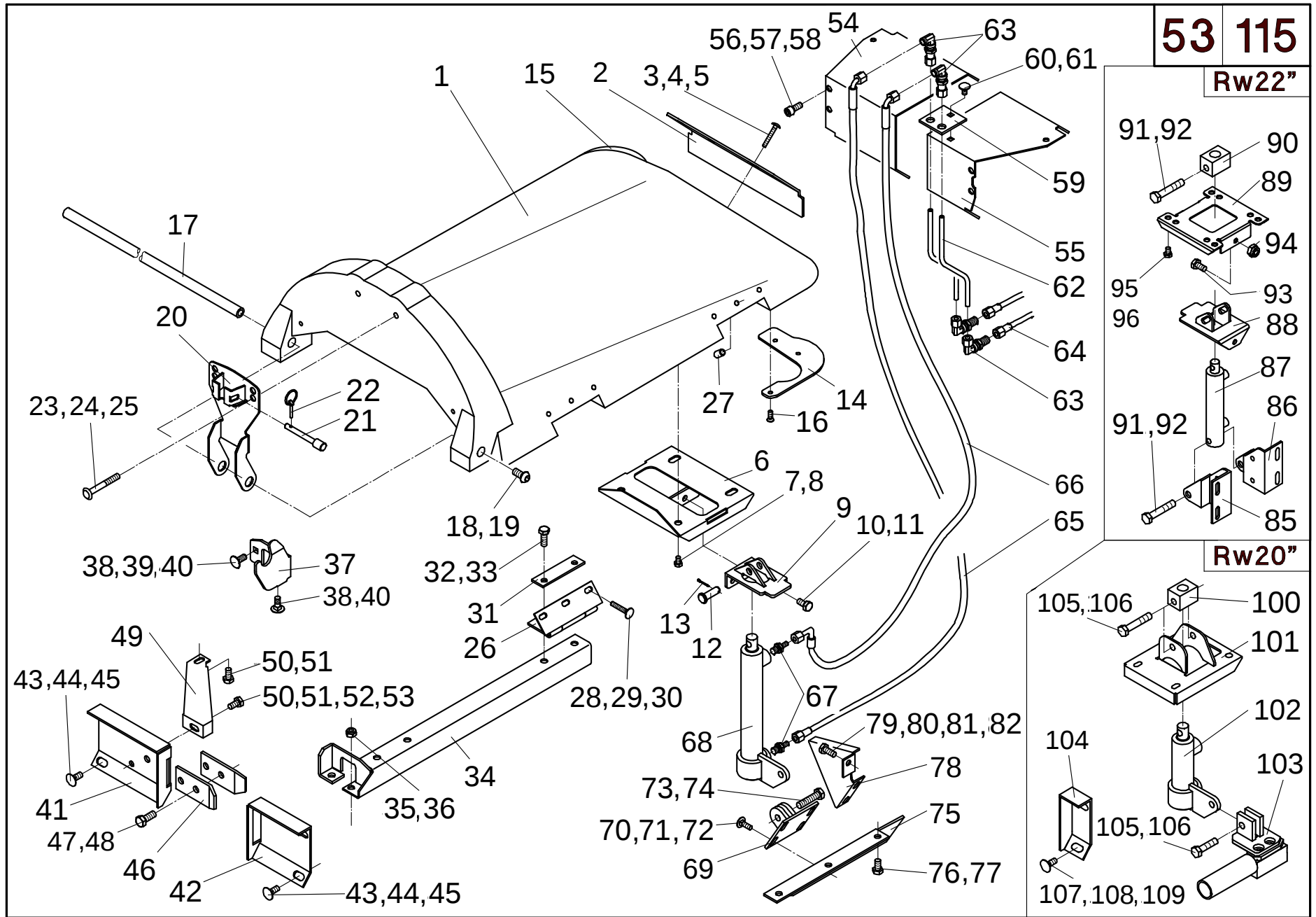
Bonnets Folding Rows 22 to 30" Rows Poly
