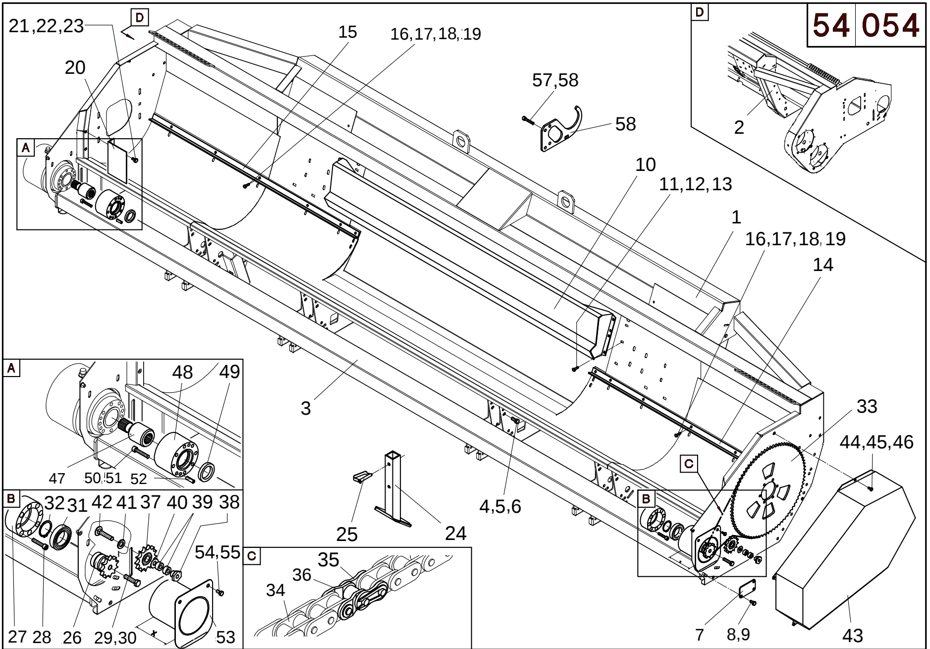
Frame 4 Row 30" to 6 Row 30" Rigid Headers
