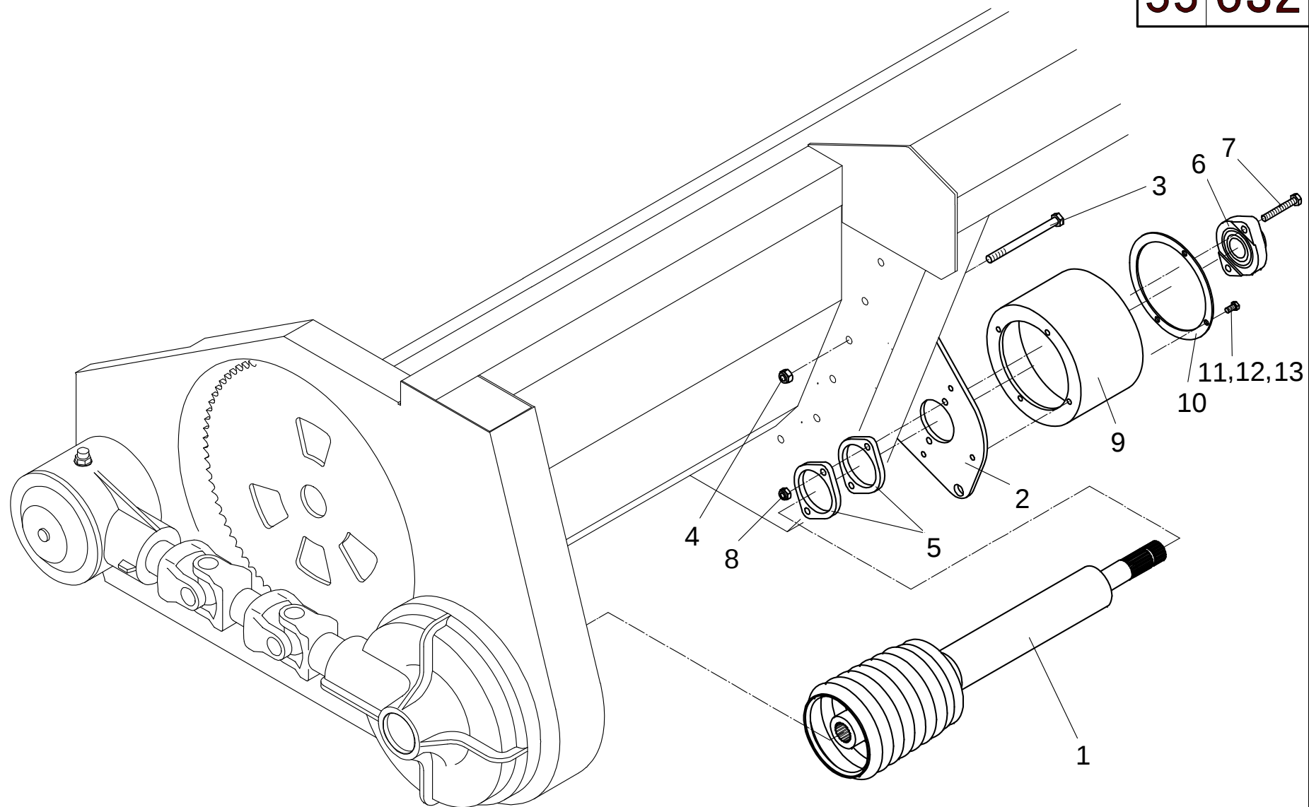
Header Drive Intermediate Shafts 836 to 1222
